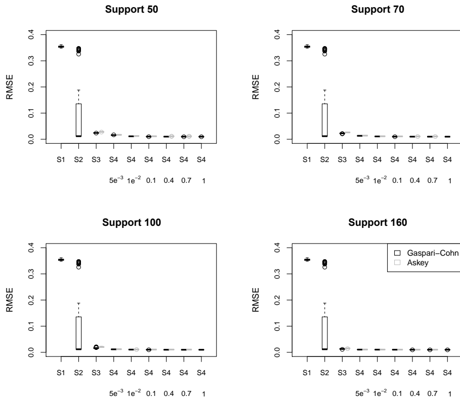
Figure 9. Same as Fig. 5 but for 500 ensemble members.
