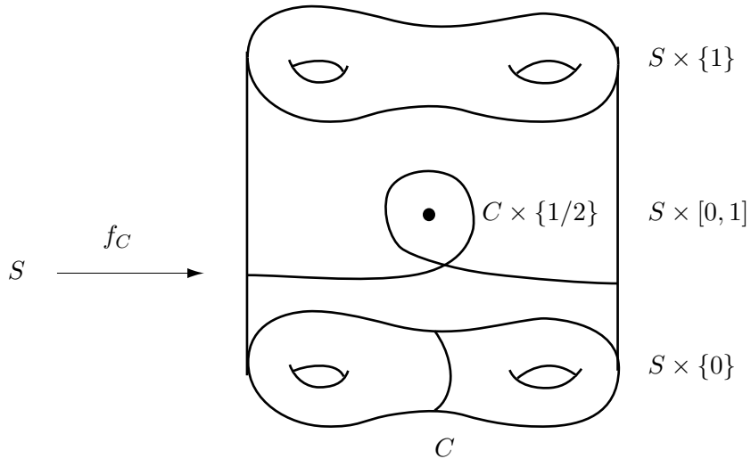
Figure 1: The wrapping map f_C .
