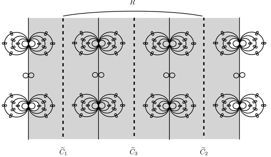
Figure 3: \Lambda(\widehat{G}) and \Omega_0(G_\infty) (the shaded part).
